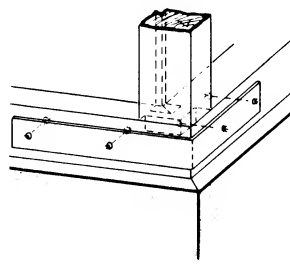
3 Corner stiffening with metal anchor
